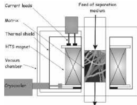
Fig. 1. HTS magnet operation scheme for HGMS
